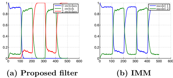
Figure 8. Probabilities of number of switches and IMM mode probabilities, underestimated r_{\max} .
