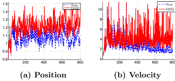
Figure 4. Normalized estimation errors of the new filter and IMM, Monte Carlo evaluation.
