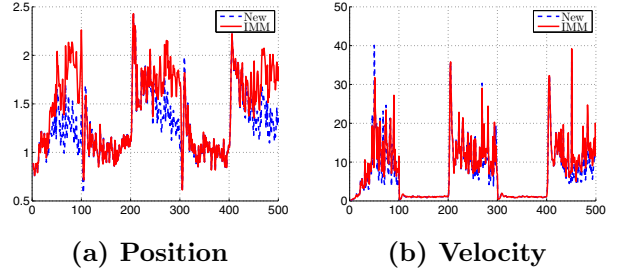
Figure 5. Normalized estimation errors of the new filter and IMM, overestimated r_{\max} .
