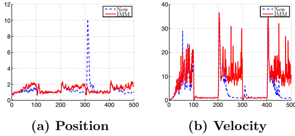
Figure 7. Normalized estimation errors of the new filter and IMM, underestimated r_{\max} .
